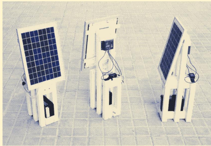
Image: a solar panel with charge controller and lead-acid battery. Photo by Marie Verdel. ☒
